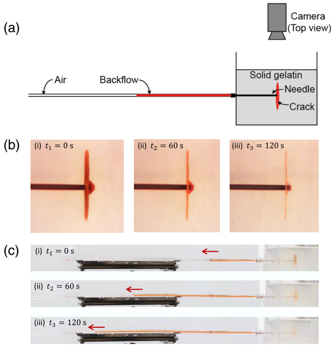
FIG. 1. (a) Schematic of the experimental setup. Representative experimental views from the (b) top and (c) side are shown. Experimental parameters: mineral oil (dye in red) viscosity \mu = 26.9 mPa s, gelatin Young's modulus E = 79 kPa, and the initial crack radius R = 21 mm. (b) The shape of the liquid-filled crack at different times as the elastic solid relaxes. (c) The propagation of liquid (dyed red) from the crack toward the open end of the tube (backflow), with the red arrows above the liquid fronts indicating the flow direction.
