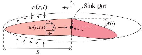
FIG. 2. Schematic of the fluid flow in a crack of radius R and half maximum thickness W(t) in an elastic reservoir during the backflow process. The elastic pressure p(r,t) surrounding the crack drives the fluid to flow towards the center and drain out of the crack with a volumetric flow rate Q(t) .
